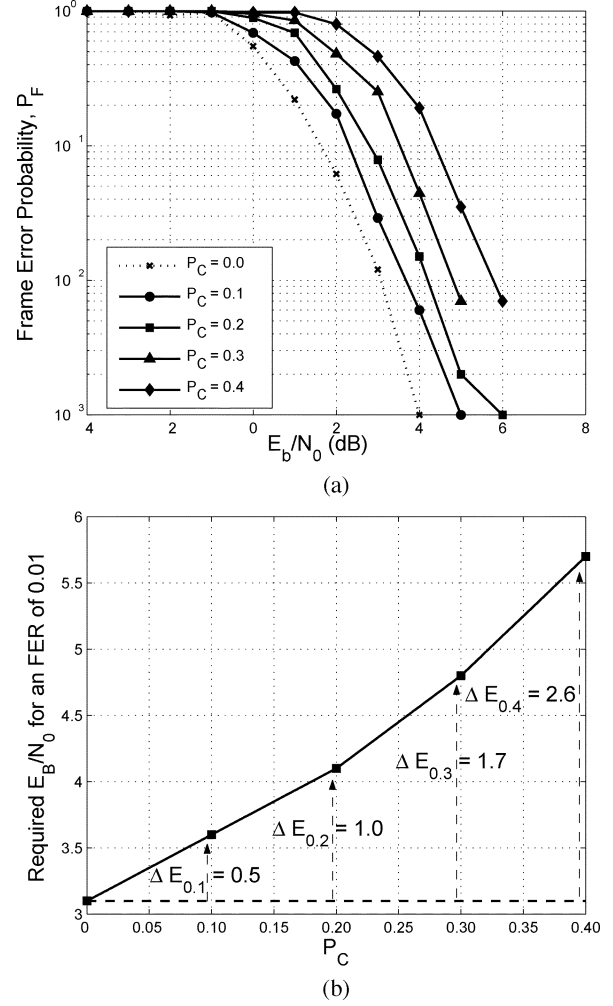
Fig. 7. FER performance of HFH-OFDMA ( N_u > N_a ). As the HP collision probability ( P_C ) increases, the HFH-OFDMA system needs additional required energy ( \Delta E ) to satisfy an FER requirement of 0.01. (a) FER curve. (b) Required E_b/N_0 and \Delta E for an FER of 0.01.
