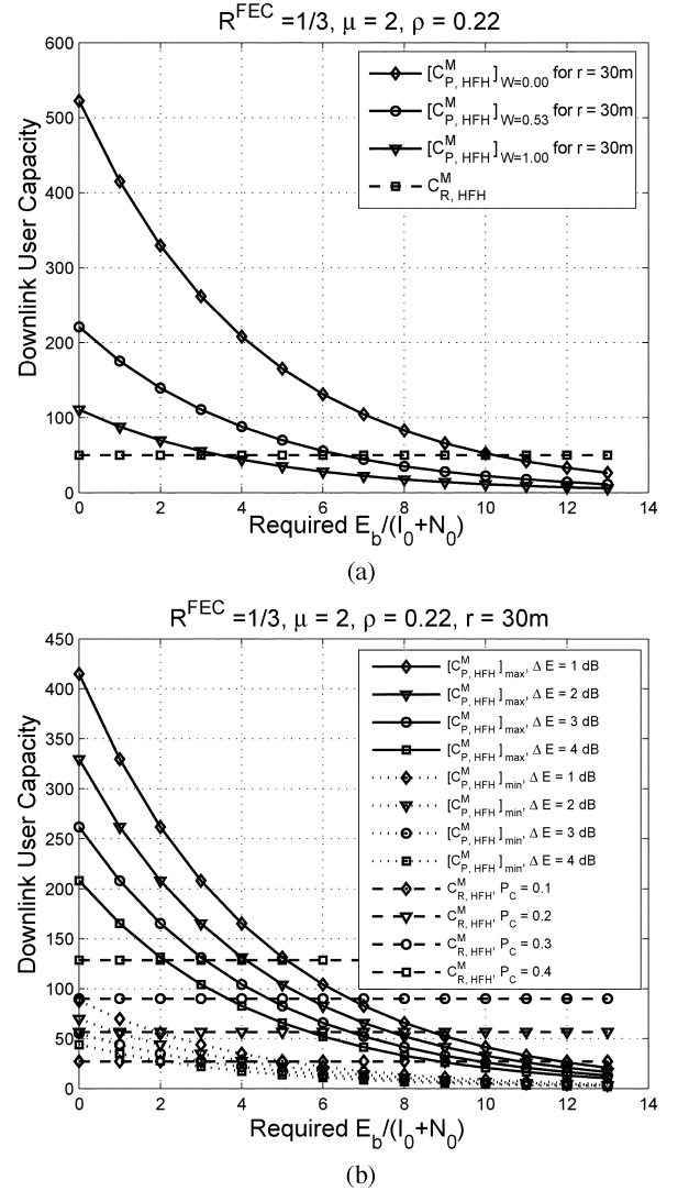
Fig. 4. Maximum and minimum downlink user capacities of the HFH-OFDMA system in the multipiconet environment. C_{P,\text{HFH}}^M decreases although C_{R,\text{HFH}}^M remains constant as the interference loading factor W increases. (a) Downlink user capacity ( N_u \leq N_a ). (b) Downlink user capacity ( N_u > N_a ).
